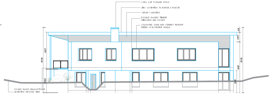
NORTH ELEVATION
