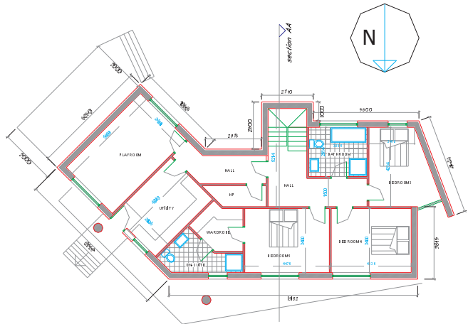
GROUND FLOOR LEVEL AREA: 125 m 2
